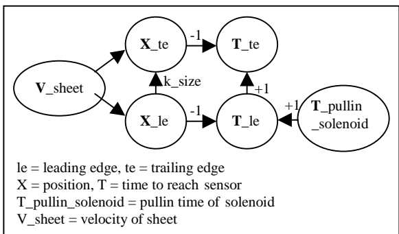
Fig. 5.2. TCG of paper path
