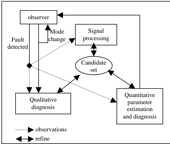
Fig. 2. Overall diagnosis architecture
