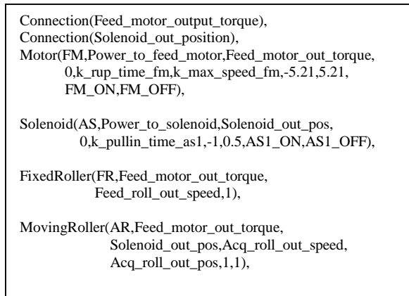
Fig. 4. Composing system model in HCC
